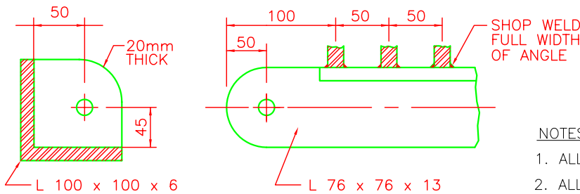
PIVOT DETAIL
